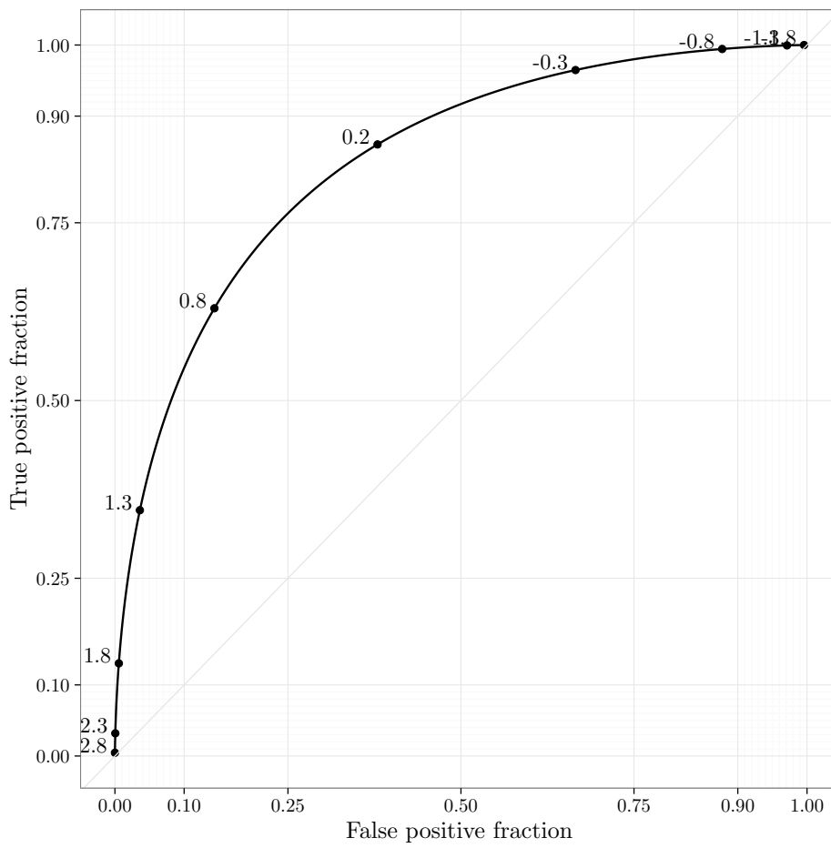
Figure 7: Illustration of smooth binormal ROC curve.
